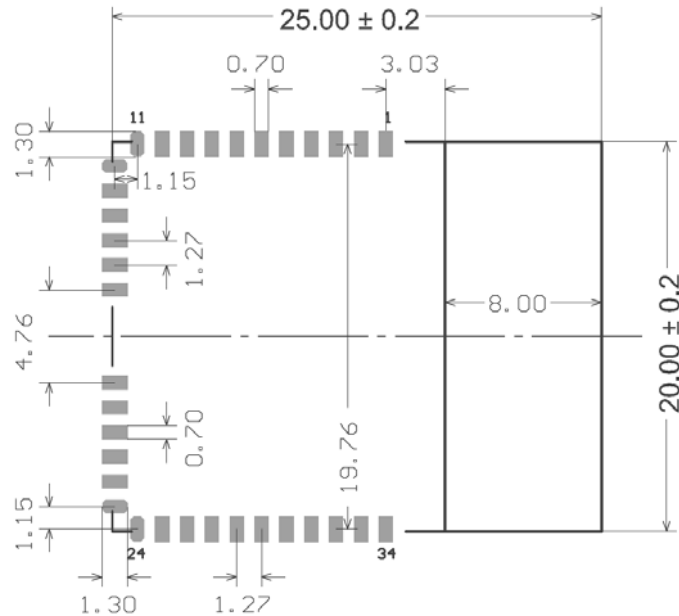
Figure 3-3: Footprint
